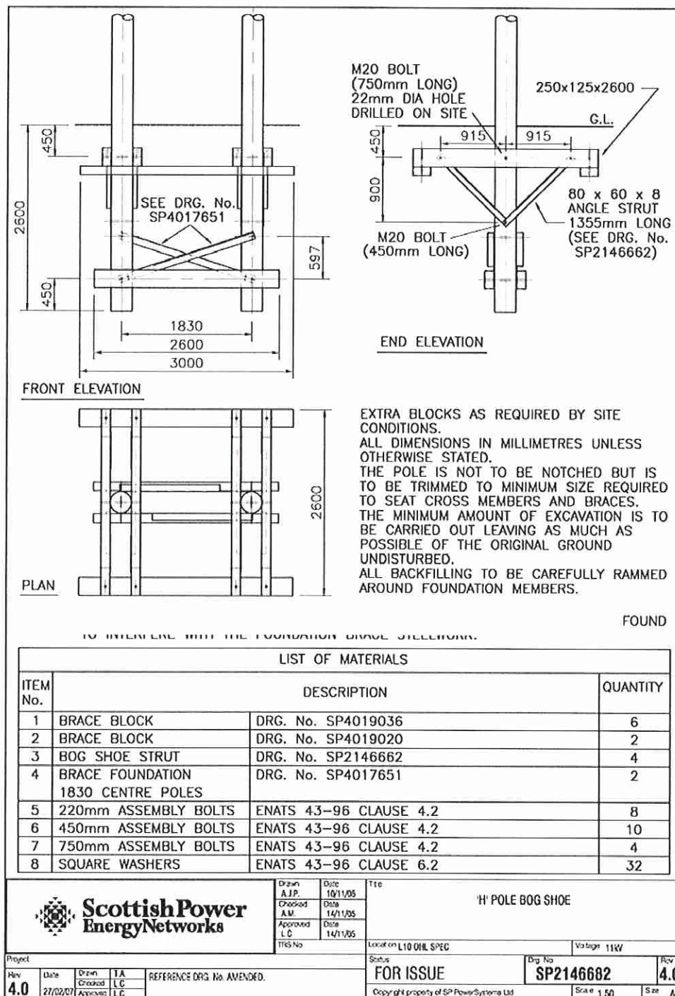
Figure 54 General Arrangement "H" Pole Bog Shoe (Drawing SP
